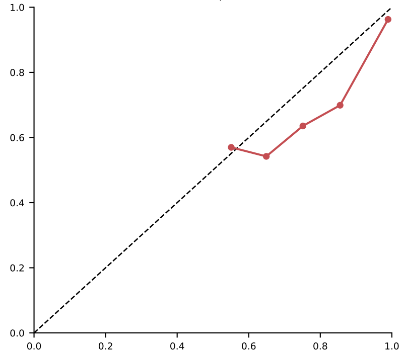
Clustered ECE=0.038, n=6846
