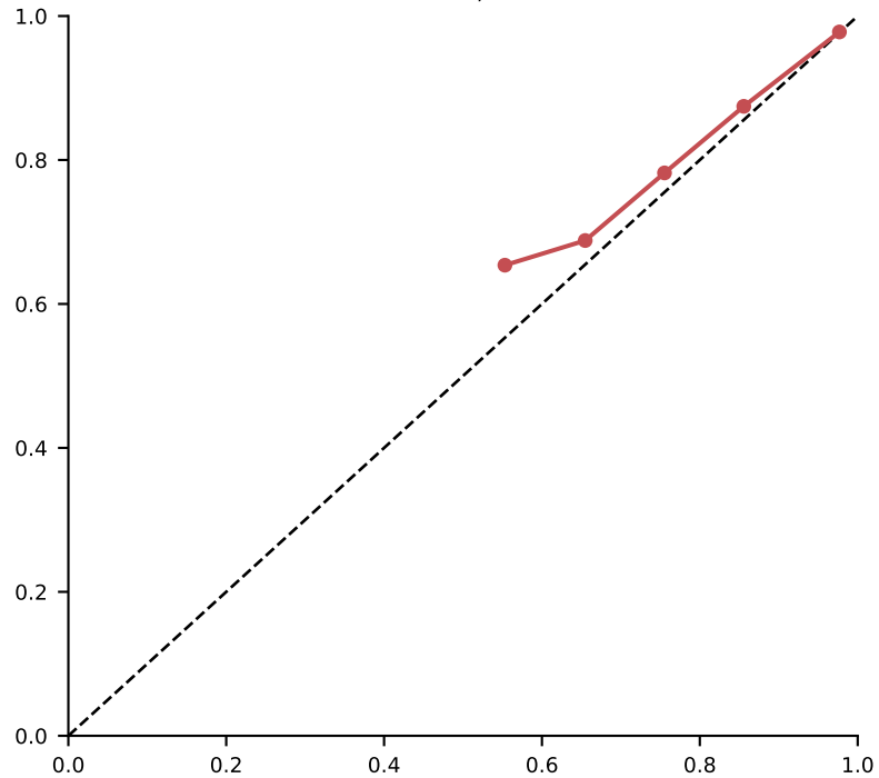
Unclustered ECE=0.007, n=6065
